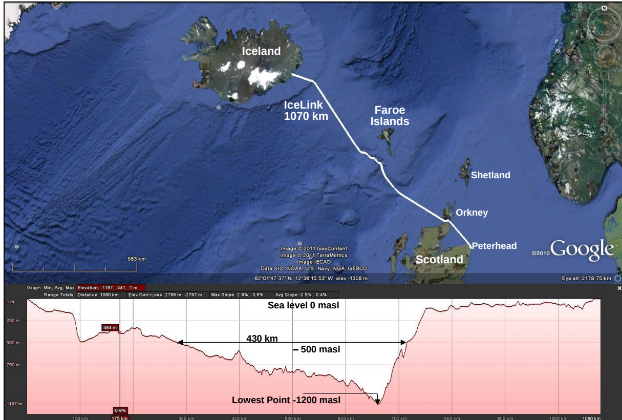
Figure 3.2 IceLink submarine cable
