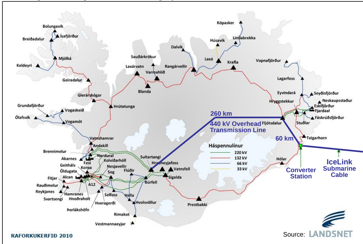
Figure 3.1 Proposed transmission projects in Iceland in connection with IceLink
