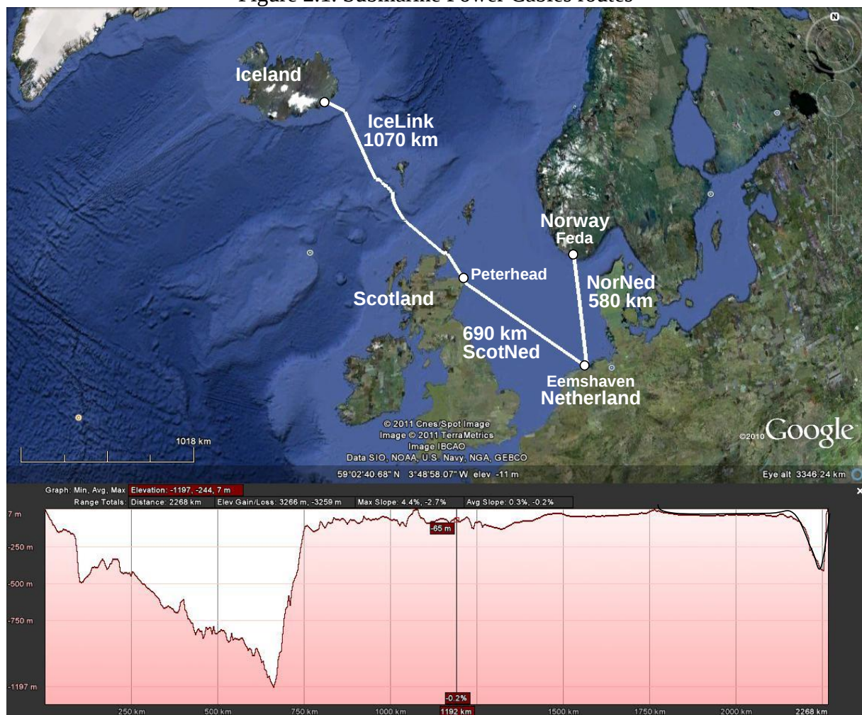
Figure 2.1. Submarine Power Cables routes
