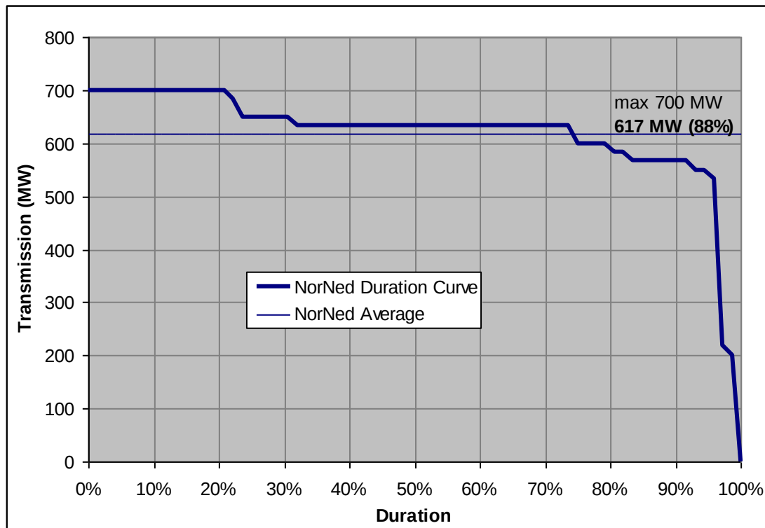
Figure 7.2. NorNed Transmission
