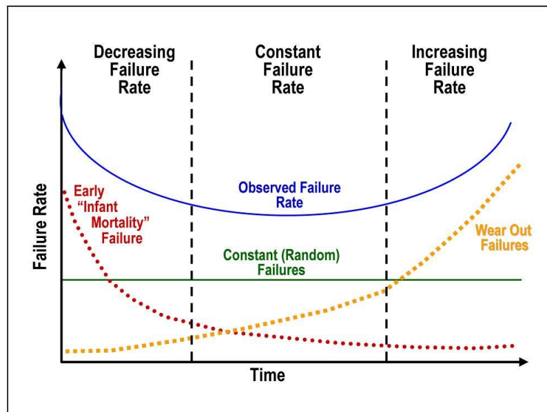
Figure 6.1. The bathtub curve
