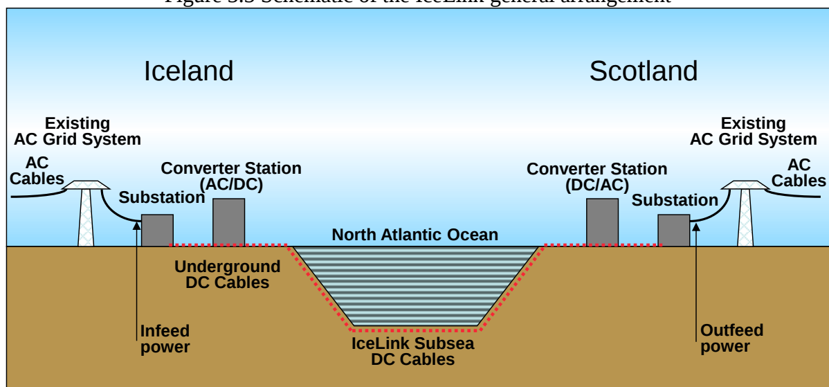
Figure 3.3 Schematic of the IceLink general arrangement
